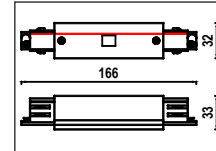
RPCTTPSC0165032B 0 ▶ MV3 Straight Coupler
