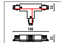
RPCTTPTC0165100B 0 ▶ MV3 T Coupler Left 37.2 ▶ MV3 T Coupler Right
