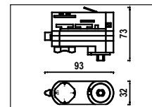
40. ▶ MV3 Spot Adaptor
