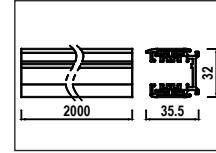
TKMV32M0000000000 0 ▶ MV3 Track Length = 2meter
